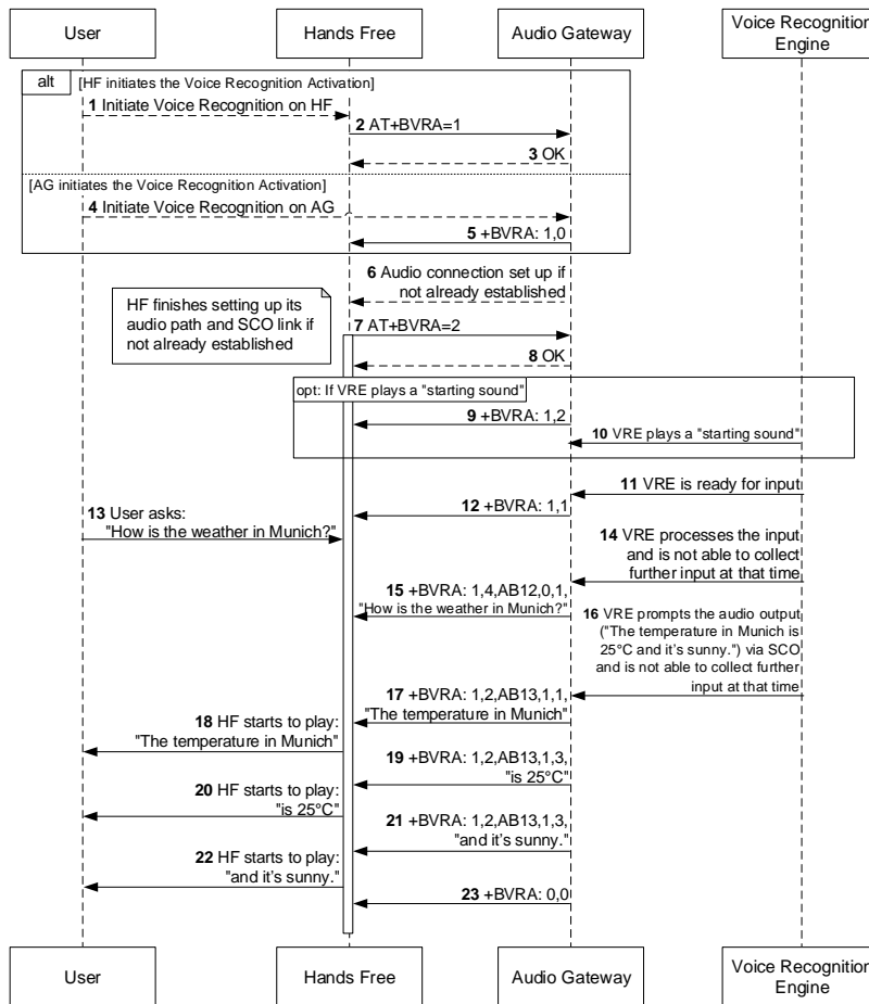
Figure 4.47: Sequence diagram with textual representation
