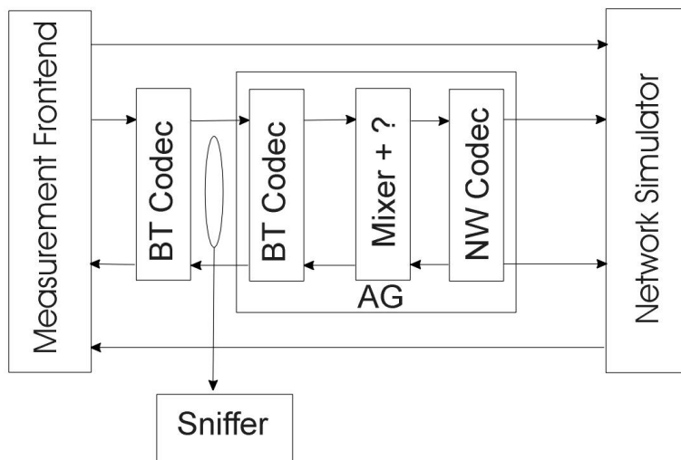
Figure 12.1: Example setup for audio level testing
